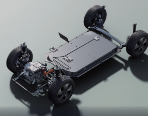
Cell To Body battery-integrated chassis
